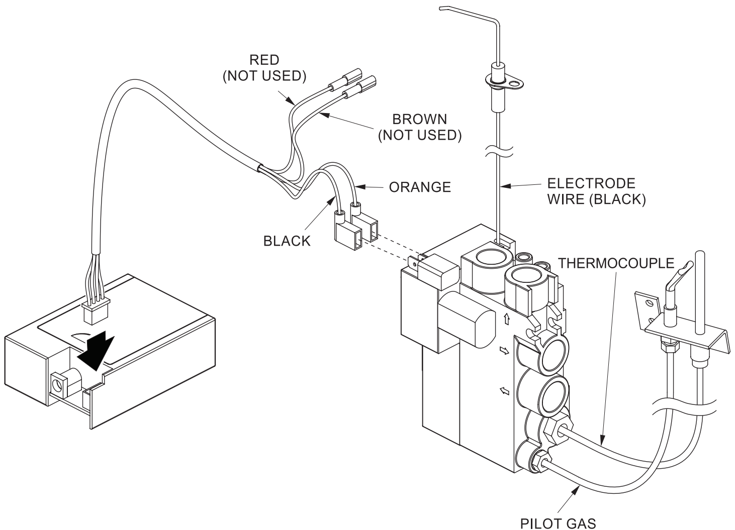
Wiring Diagram Figure 13
