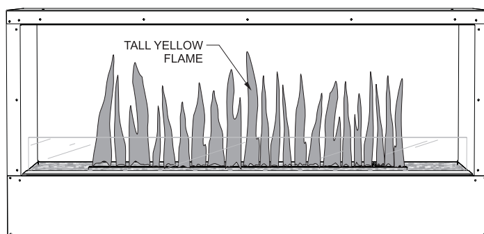
Figure 34 - Incorrect Tall Yellow Flame
