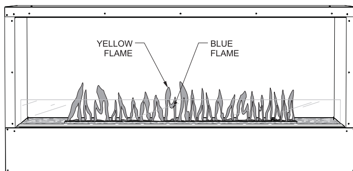
Figure 32 - Correct Flame Natural
