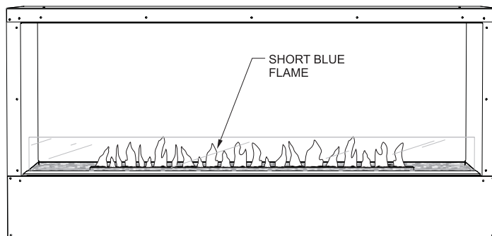
Figure 33 - Incorrect Short Blue Flame
