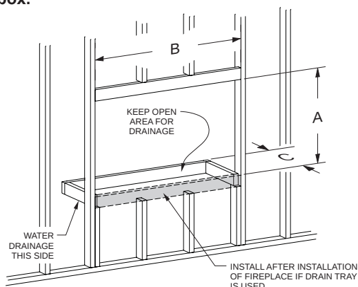
FRAMING DIMENSIONS (in inches)
