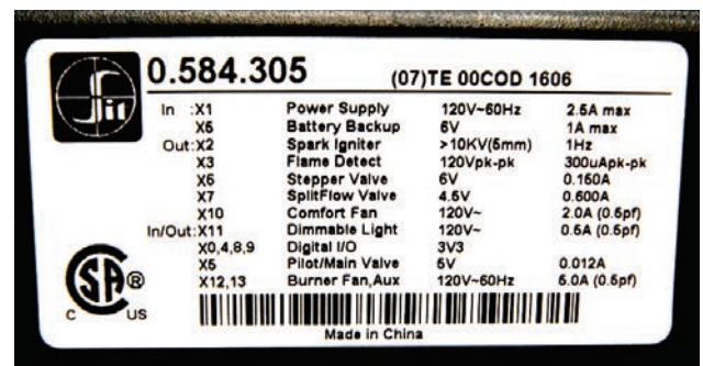
Bottom of Receiver Module
